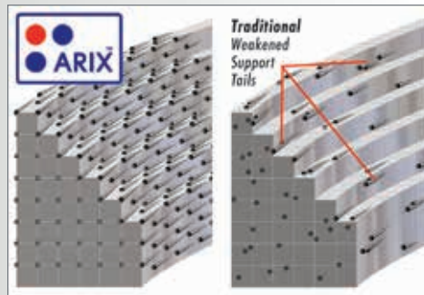
G3 ARIX™ Turbo Standard Segment
